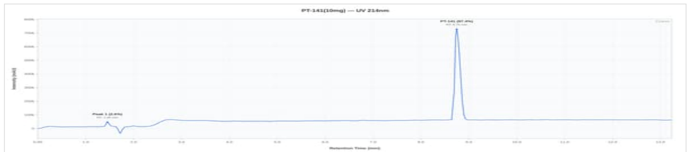
PT-141 10mg - DP-2607-01: UV Chromatogram
